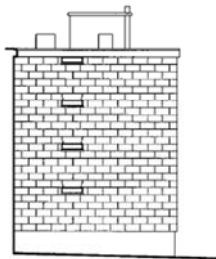
FACADE SUD
