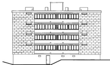
FACADE SUD
